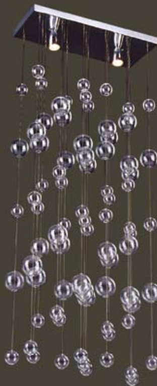
art C0129-2B 58*23*30(HxWxD) G5.3 2*20W 220V material chrome
