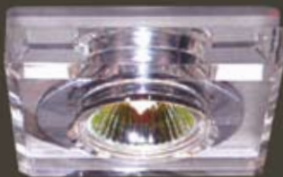
art SC529R 65*65 (HxWxD) MR16 50W 12V Material
