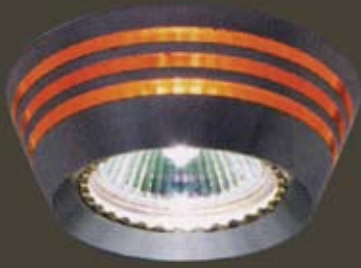
art LKC-253C 53.5*22*36.5 (HxWxD) MR16 50W 12V acrylic+aluminium
