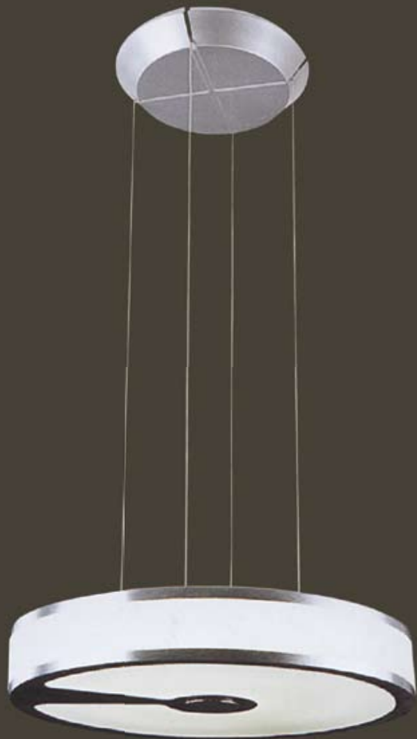
art 8655-2ROUND 53*53*16 (HxWxD) T5 1*55W 1*32W 220V material aluminum+ plastic
