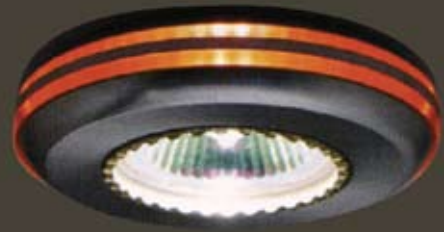
art LKC-251C (HxWxD) MR16 50W 12V acrylic+aluminium
