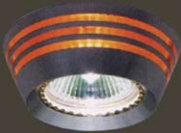
art LKC-253C 53.5*22*36.5 (HxWxD) MR16 50W 12V acrylic+aluminium
