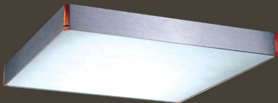
art 1558/6+1243 97*17*97 (HxWxD) T5 6*21W 230V material aluminium
